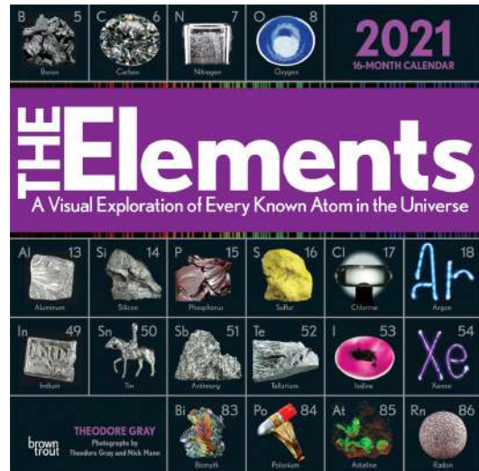
ELEMENTS, THE
