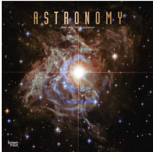
ASTRONOMY
