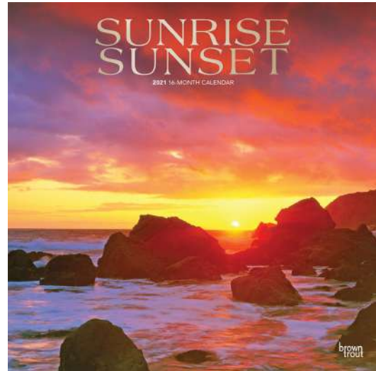
SUNRISE SUNSET
